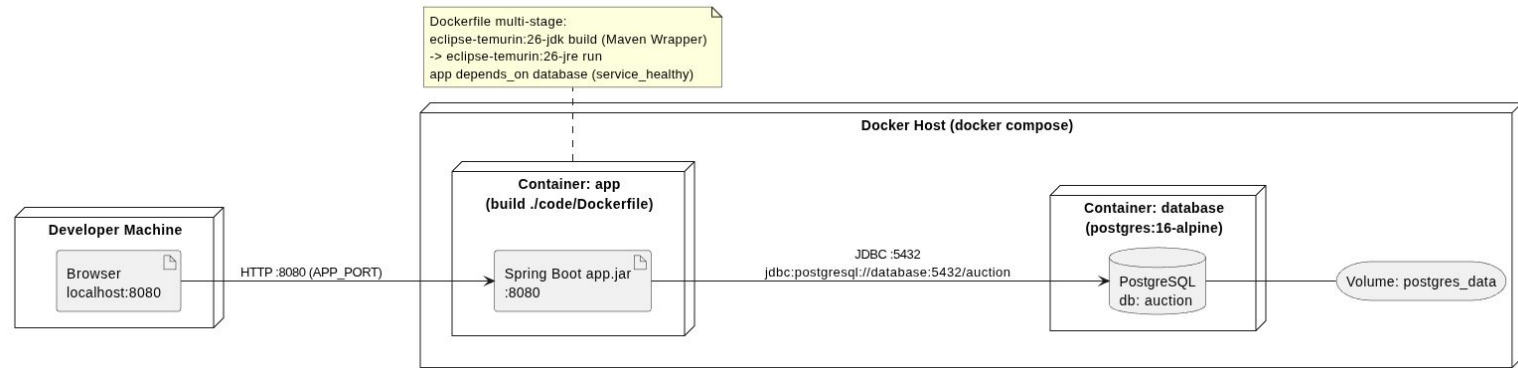
Deployment Diagram - Local (docker-compose)
