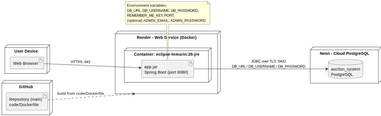
Deployment Diagram - Production (Render + Neon)
